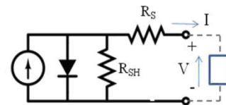
Figure2. Circuit diagram of the PV model
