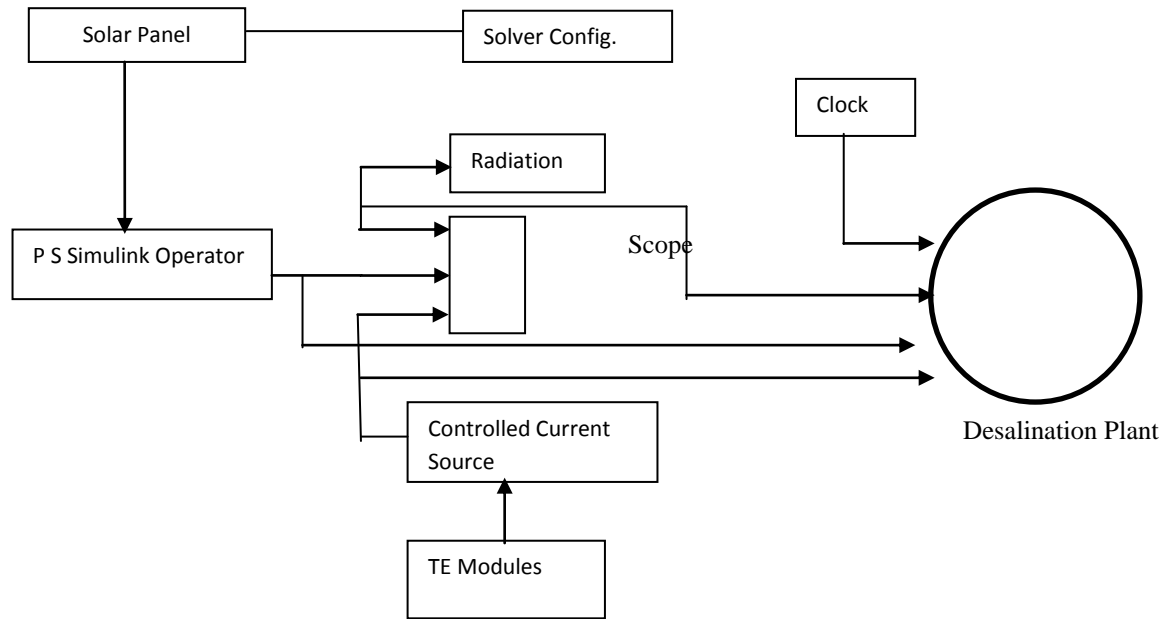
Figure. 1. Hybrid Photovoltaic and Thermoelectric Generator system for desalination
