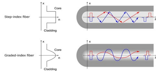
Fig.1 Graded index optical fibre
