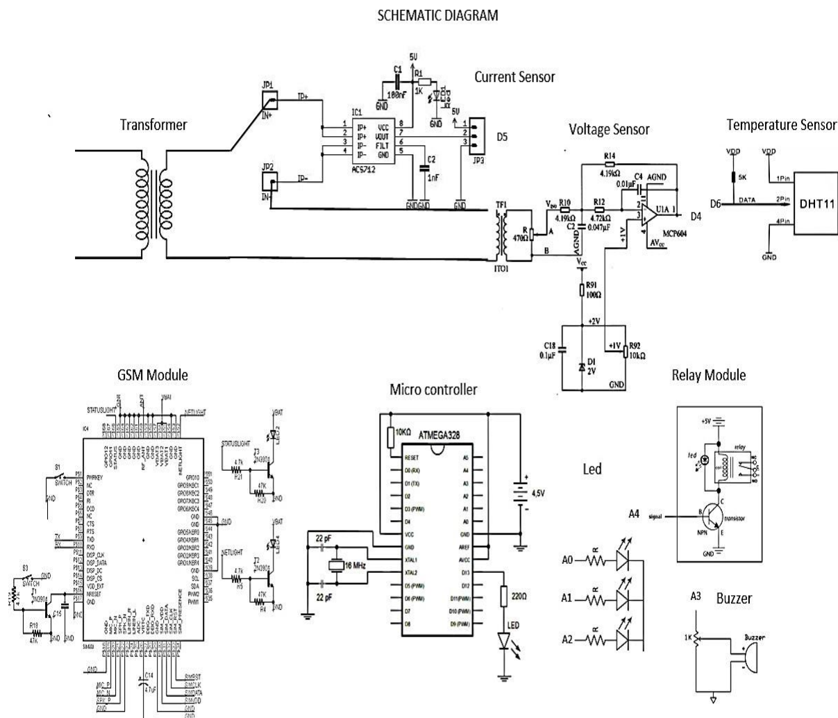
Fig.2CircuitDiagram
